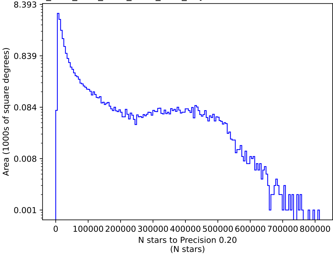
ddf_acor_sf20_lsf30_lsr20_v3.4_10yrs i: N stars to Precision 0.20
