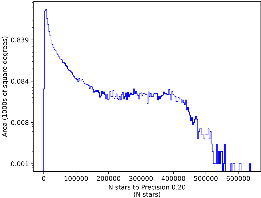
ddf_acor_sf20_lsf30_lsr20_v3.4_10yrs g: N stars to Precision 0.20
