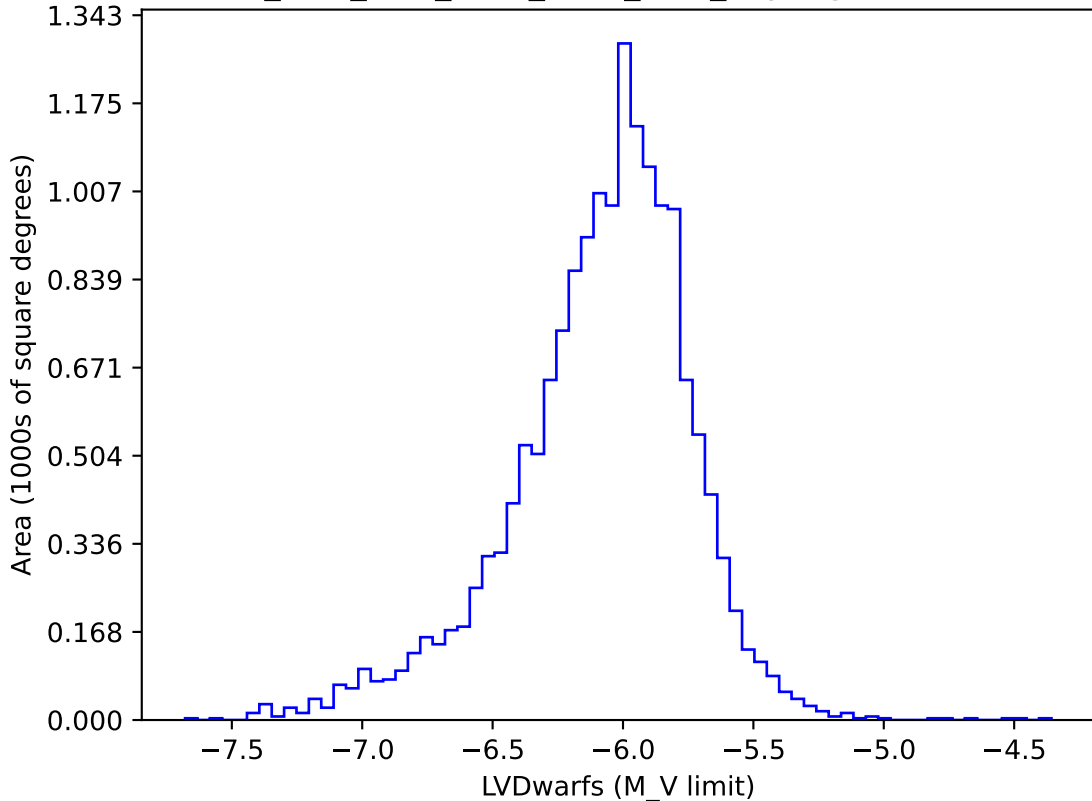
ddf_acor_sf20_lsf30_lsr20_v3.4_10yrs gi: LVDwarfs
