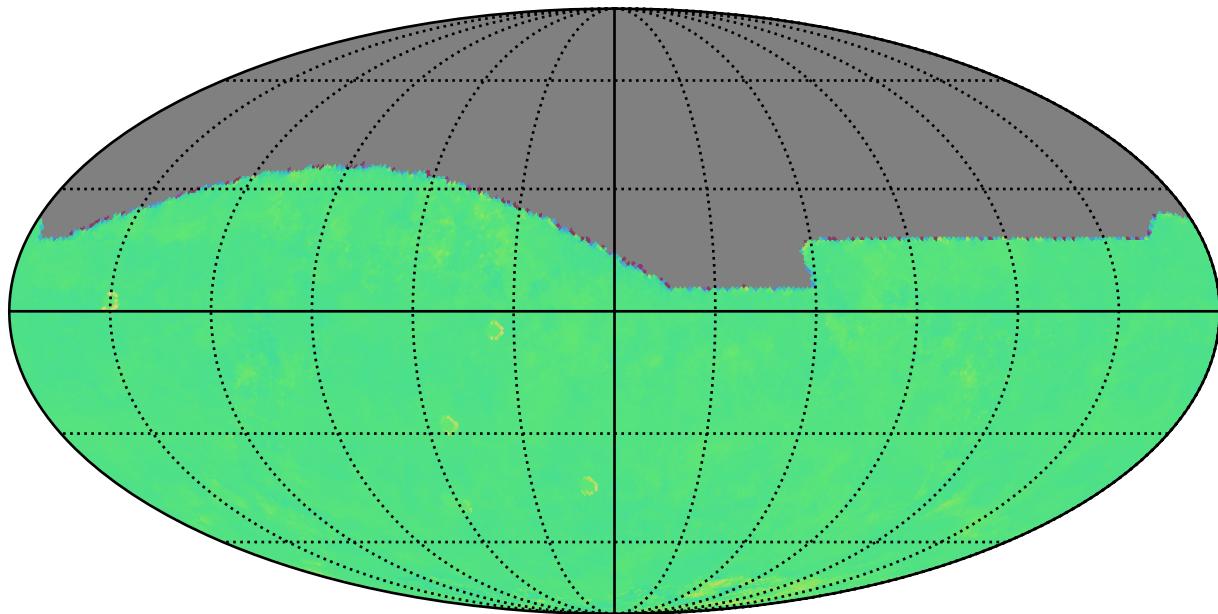
ddf_acor_sf20_lsf30_lsr20_v3.4_10yrs r: Kuiper rotTelPos
