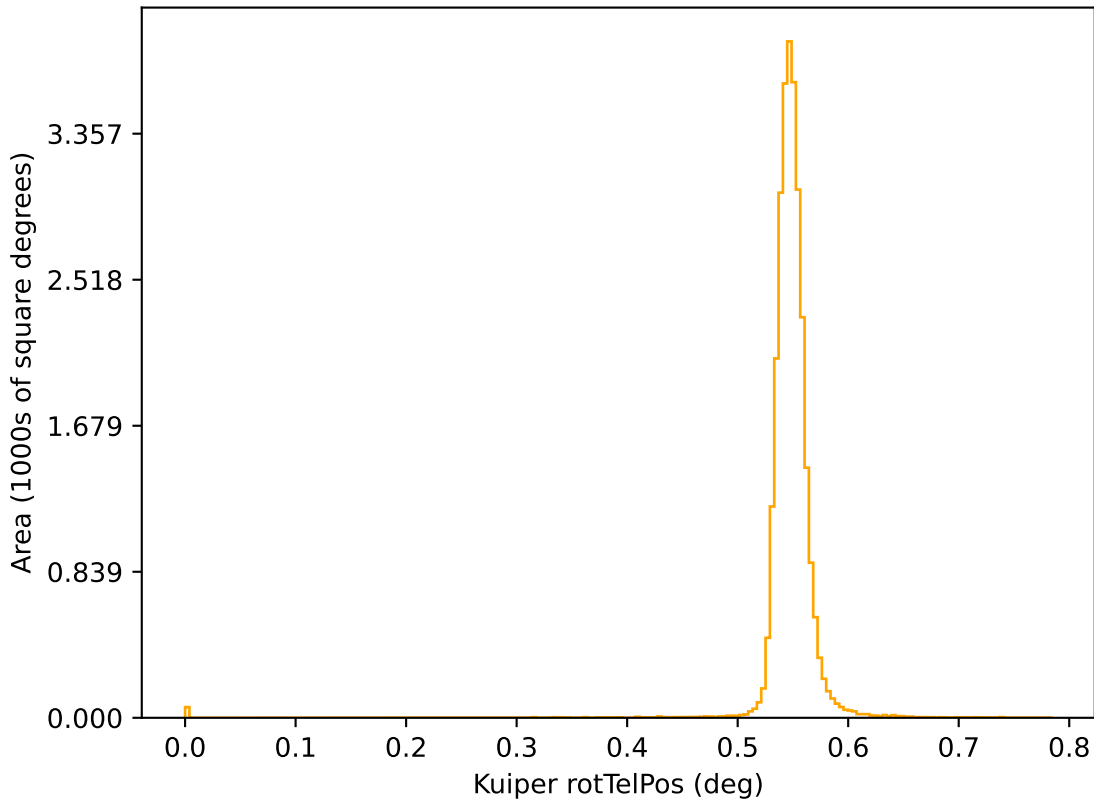
ddf_acor_sf20_lsf30_lsr20_v3.4_10yrs r: Kuiper rotTelPos
