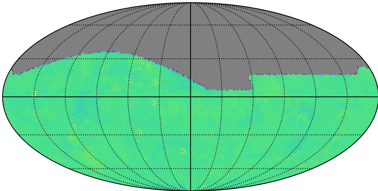
ddf_acor_sf20_lsf30_lsr20_v3.4_10yrs g: Kuiper rotTelPos
