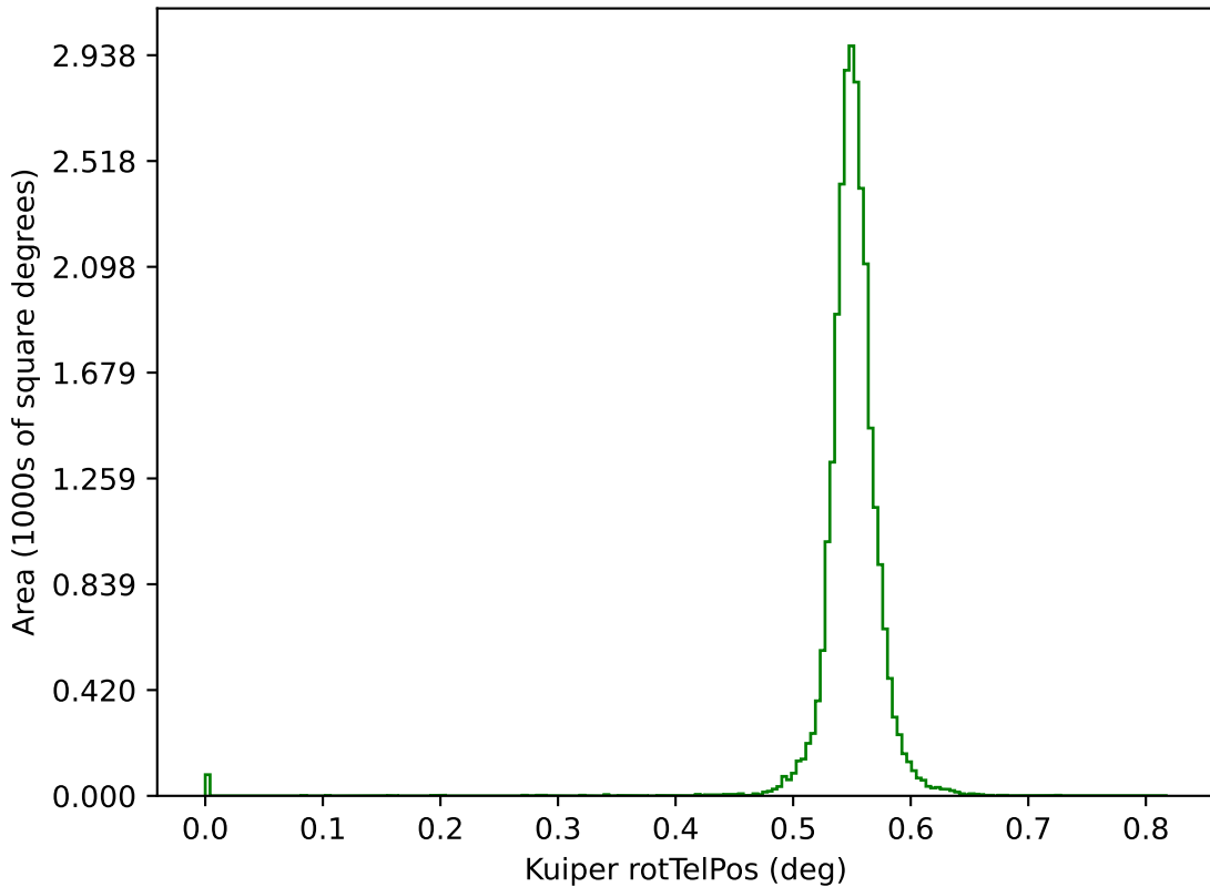
ddf_acor_sf20_ls30_lsr20_v3.4_10yrs g: Kuiper rotTelPos
