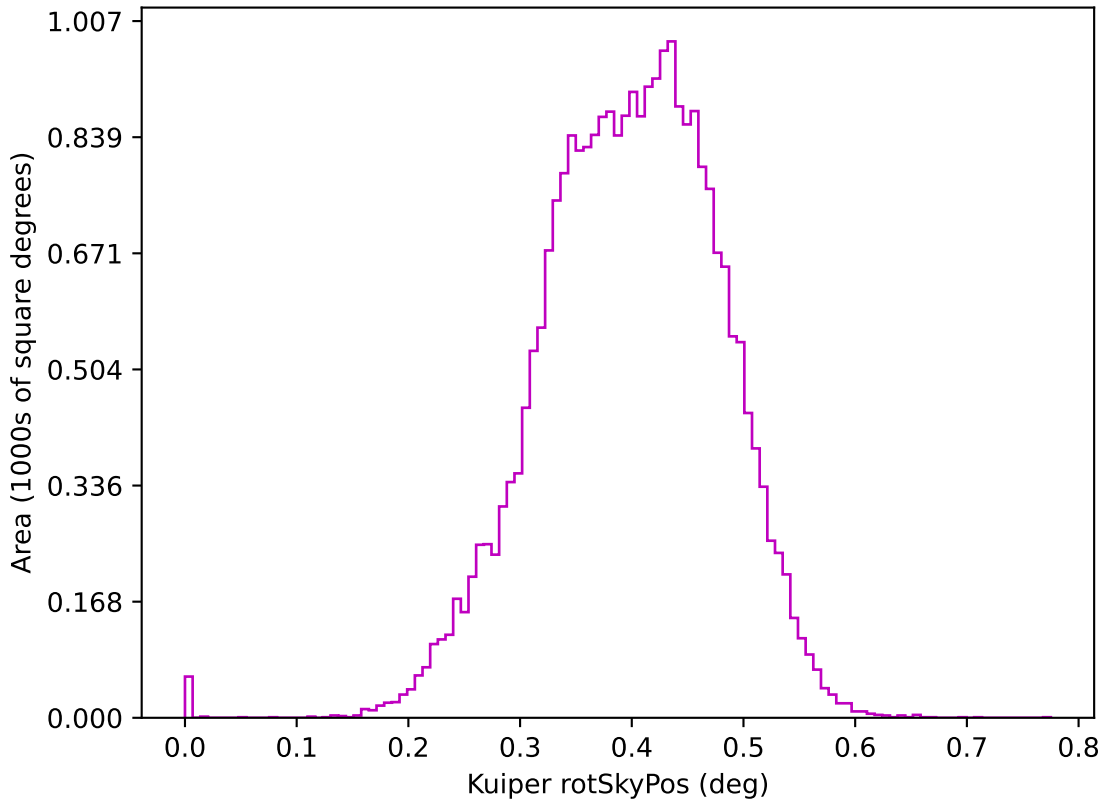
ddf_acor_sf20_lsf30_lsr20_v3.4_10yrs z: Kuiper rotSkyPos
