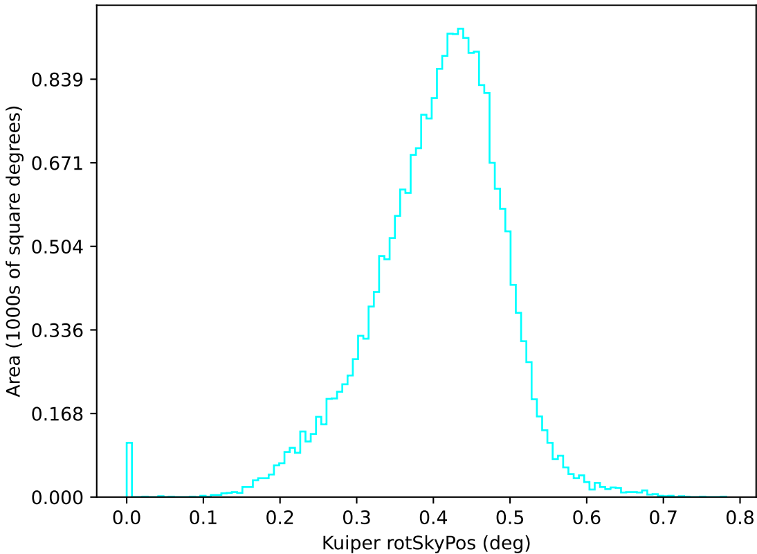
ddf_acor_sf20_lsf30_lsr20_v3.4_10yrs u: Kuiper rotSkyPos
