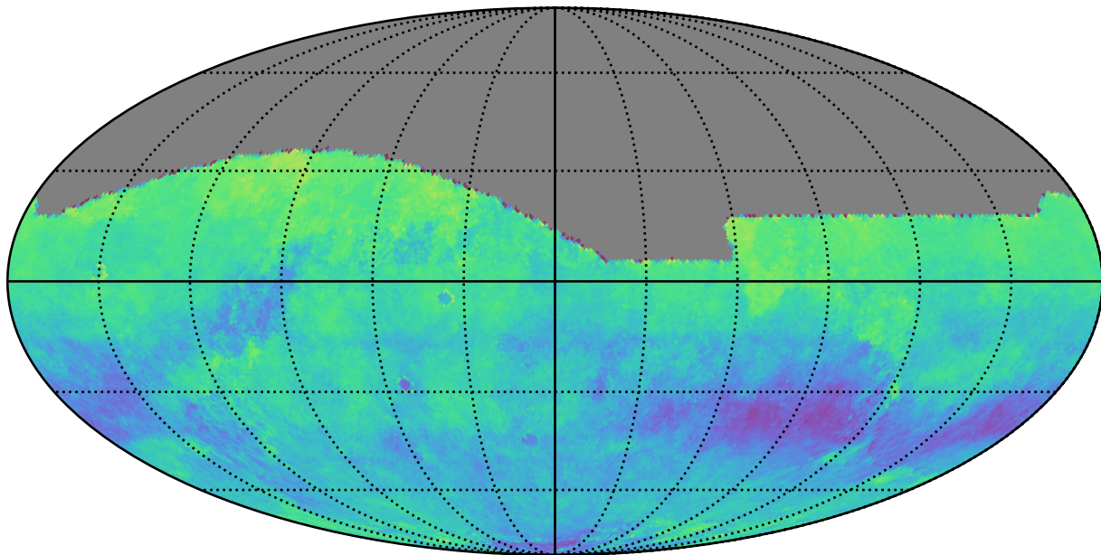
ddf_acor_sf20_lsf30_lsr20_v3.4_10yrs r: Kuiper rotSkyPos
