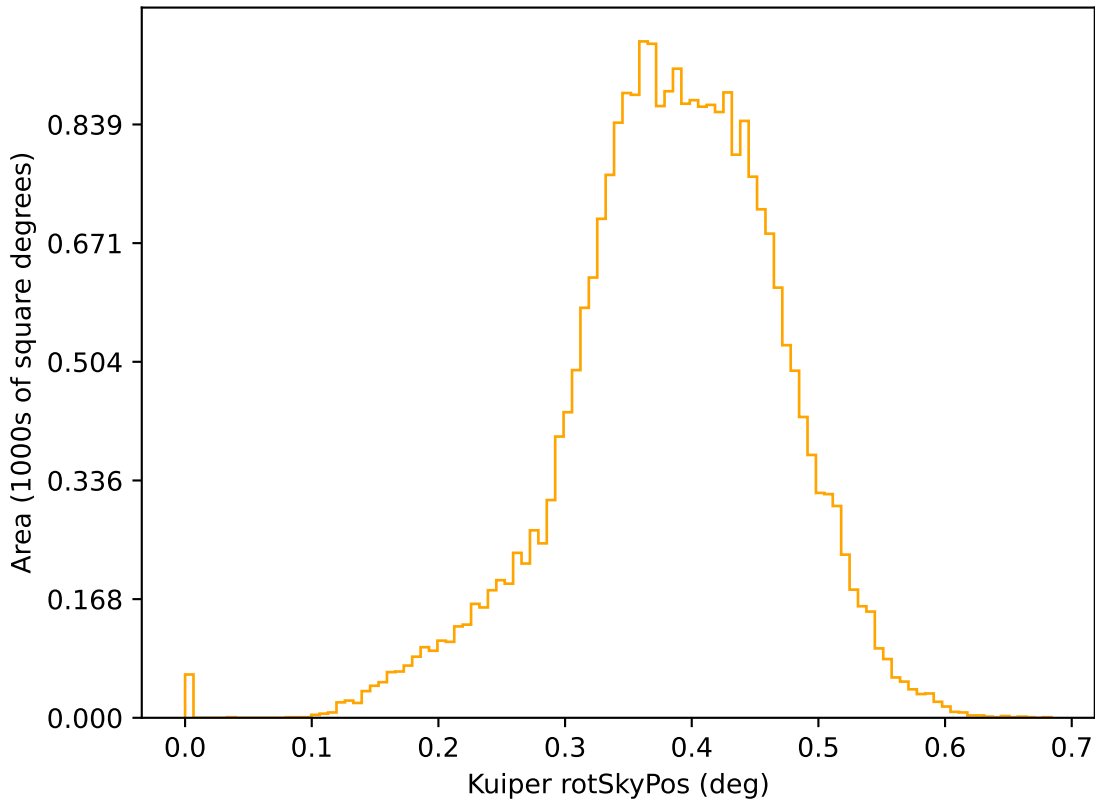
ddf_acor_sf20_lsf30_lsr20_v3.4_10yrs r: Kuiper rotSkyPos
