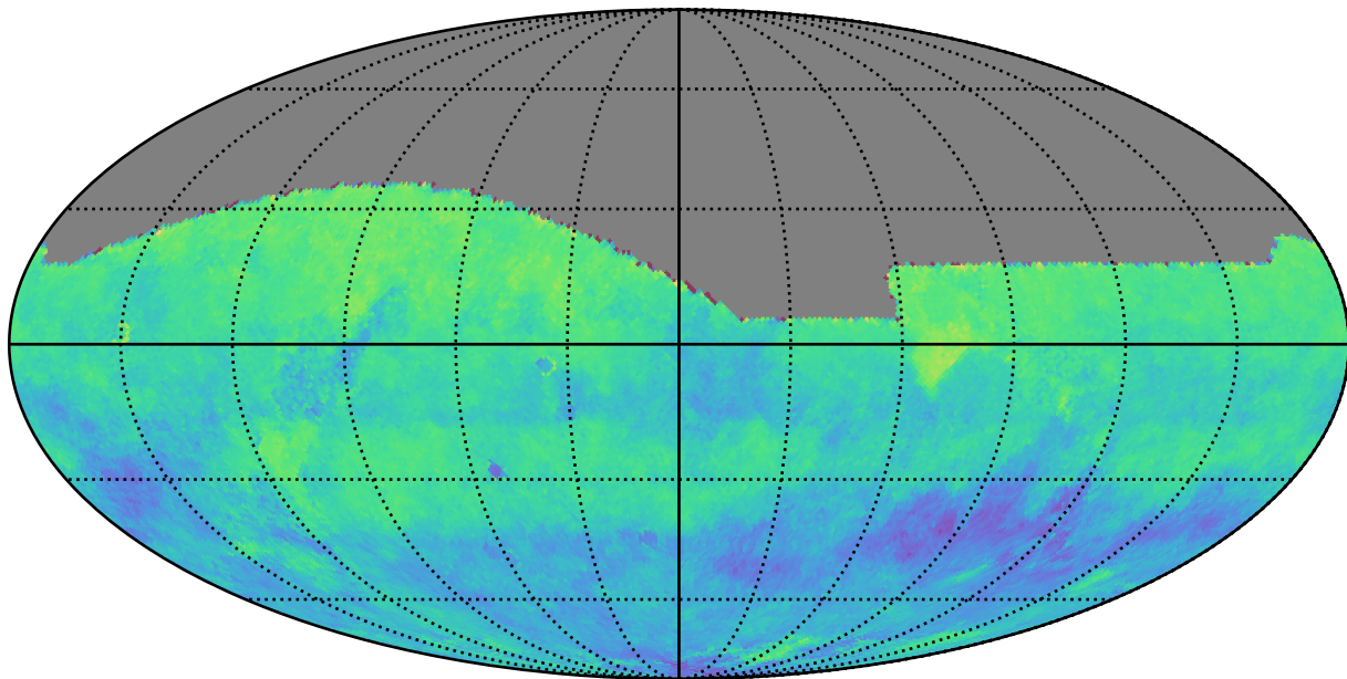
ddf_acor_sf20_lsf30_lsr20_v3.4_10yrs i: Kuiper rotSkyPos
