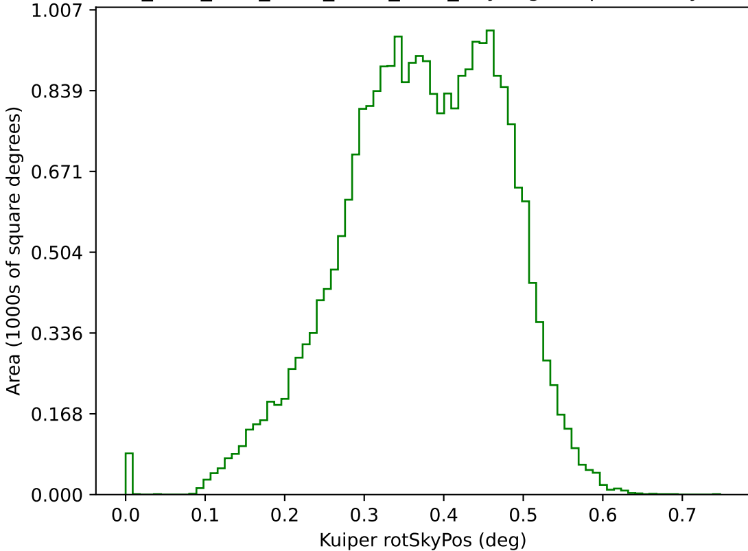
ddf_acor_sf20_lsf30_lsr20_v3.4_10yrs g: Kuiper rotSkyPos
