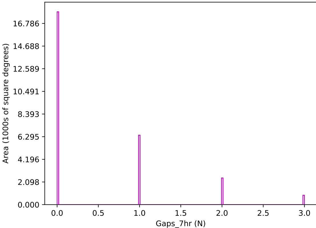
ddf_acor_sf20_ls30_lsr20_v3.4_10yrs z band: Gaps_7hr
