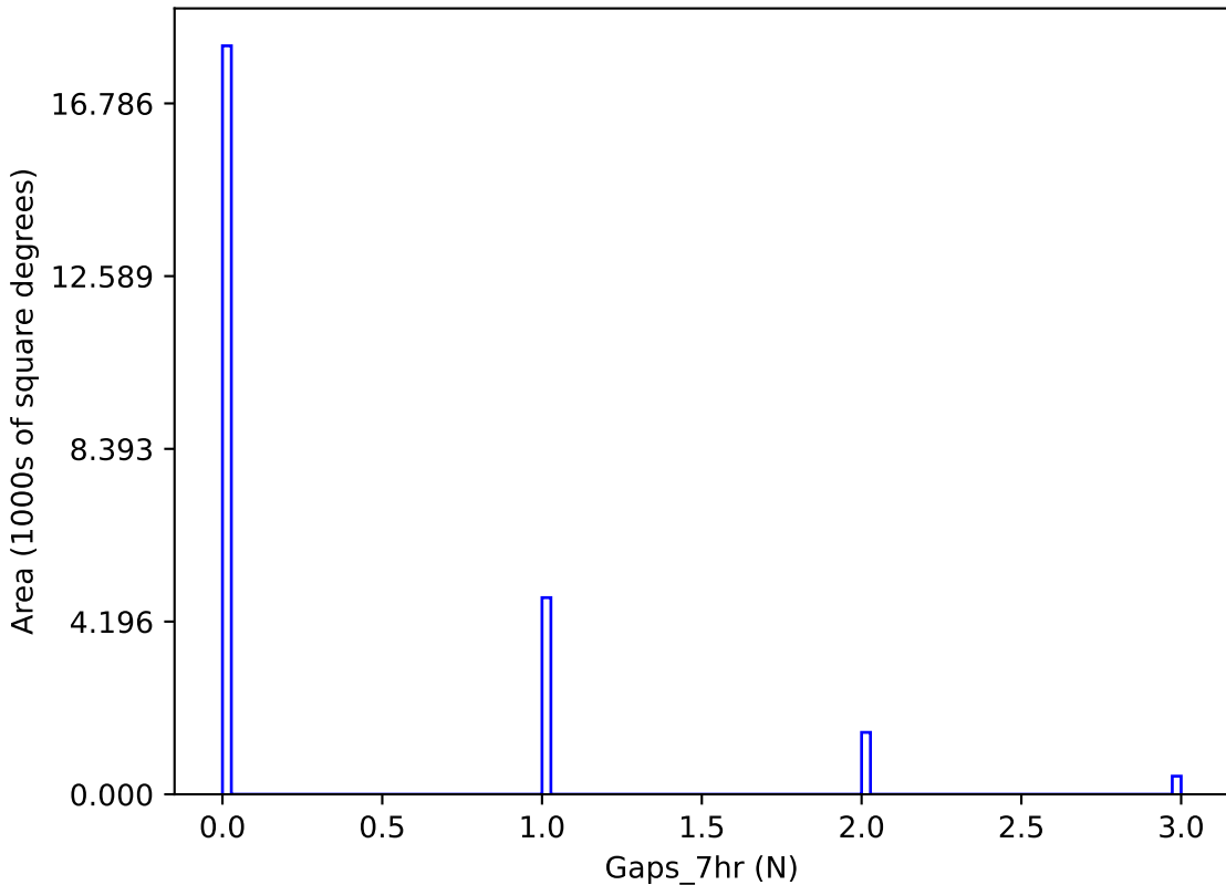
ddf_acor_sf20_lsf30_lsr20_v3.4_10yrs y band: Gaps_7hr
