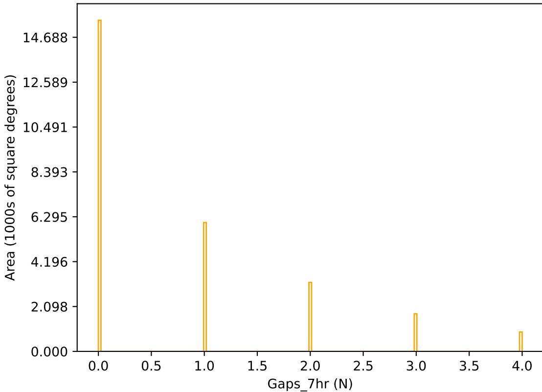
ddf_acor_sf20_lsf30_lsr20_v3.4_10yrs r band: Gaps_7hr
