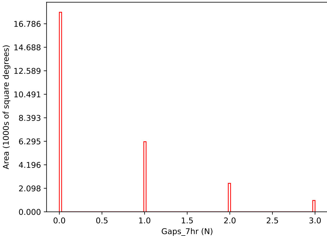
ddf_acor_sf20_lsf30_lsr20_v3.4_10yrs i band: Gaps_7hr
