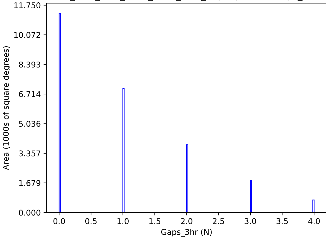
ddf_acor_sf20_lsf30_lsr20_v3.4_10yrs y band: Gaps_3hr
