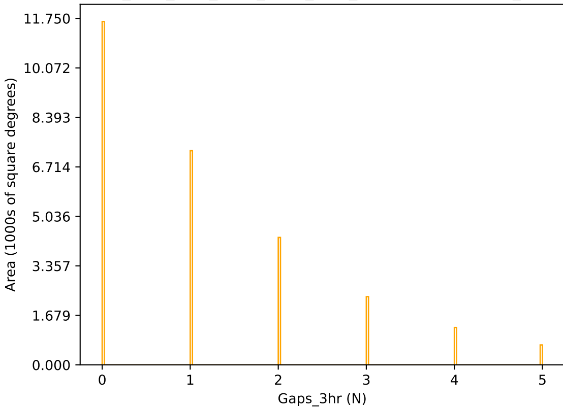
ddf_acor_sf20_lsf30_lsr20_v3.4_10yrs r band: Gaps_3hr
