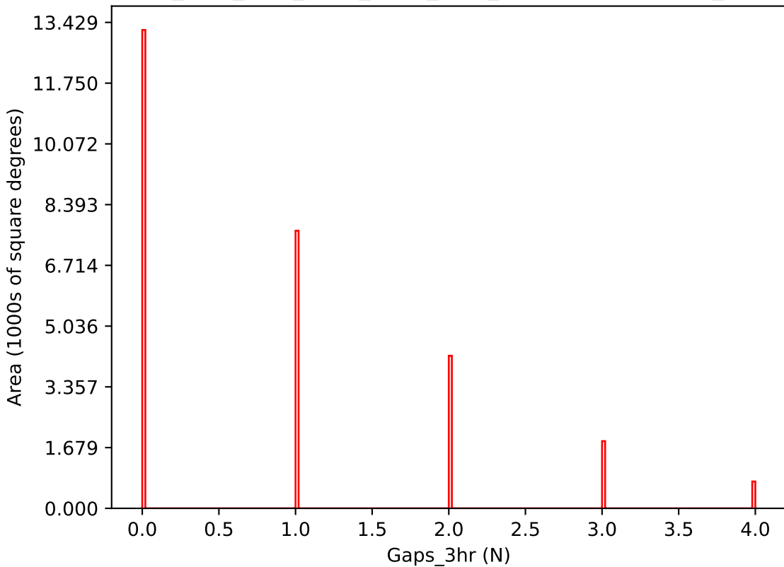
ddf_acor_sf20_lsf30_lsr20_v3.4_10yrs i band: Gaps_3hr
