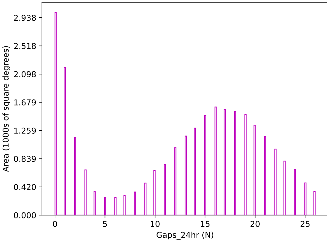
ddf_acor_sf20_lsf30_lsr20_v3.4_10yrs z band: Gaps_24hr
