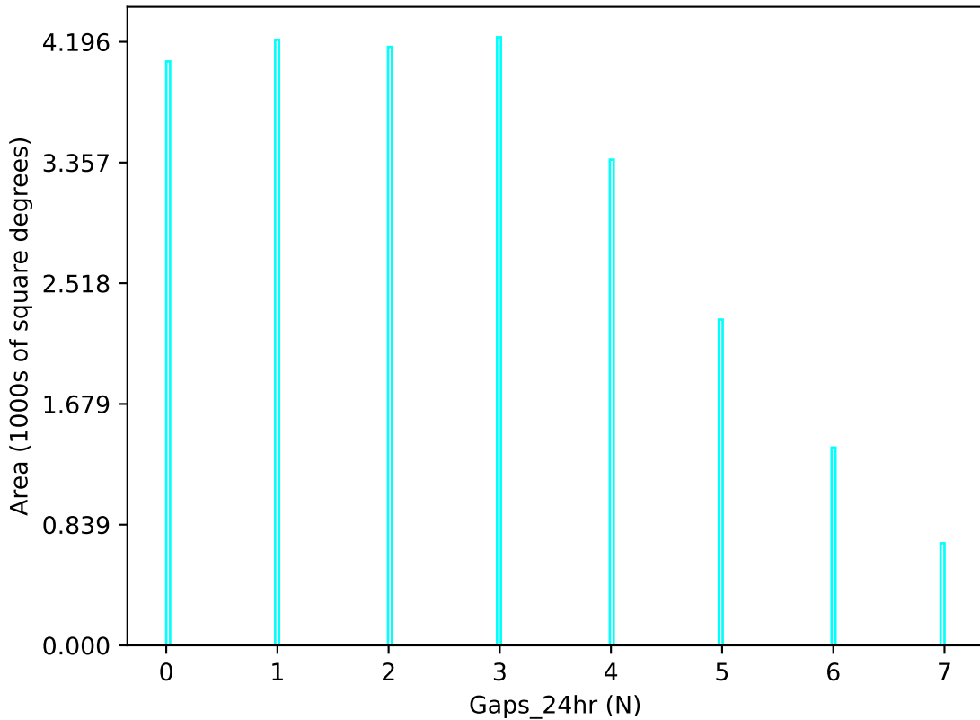
ddf_acor_sf20_lsf30_lsr20_v3.4_10yrs u band: Gaps_24hr
