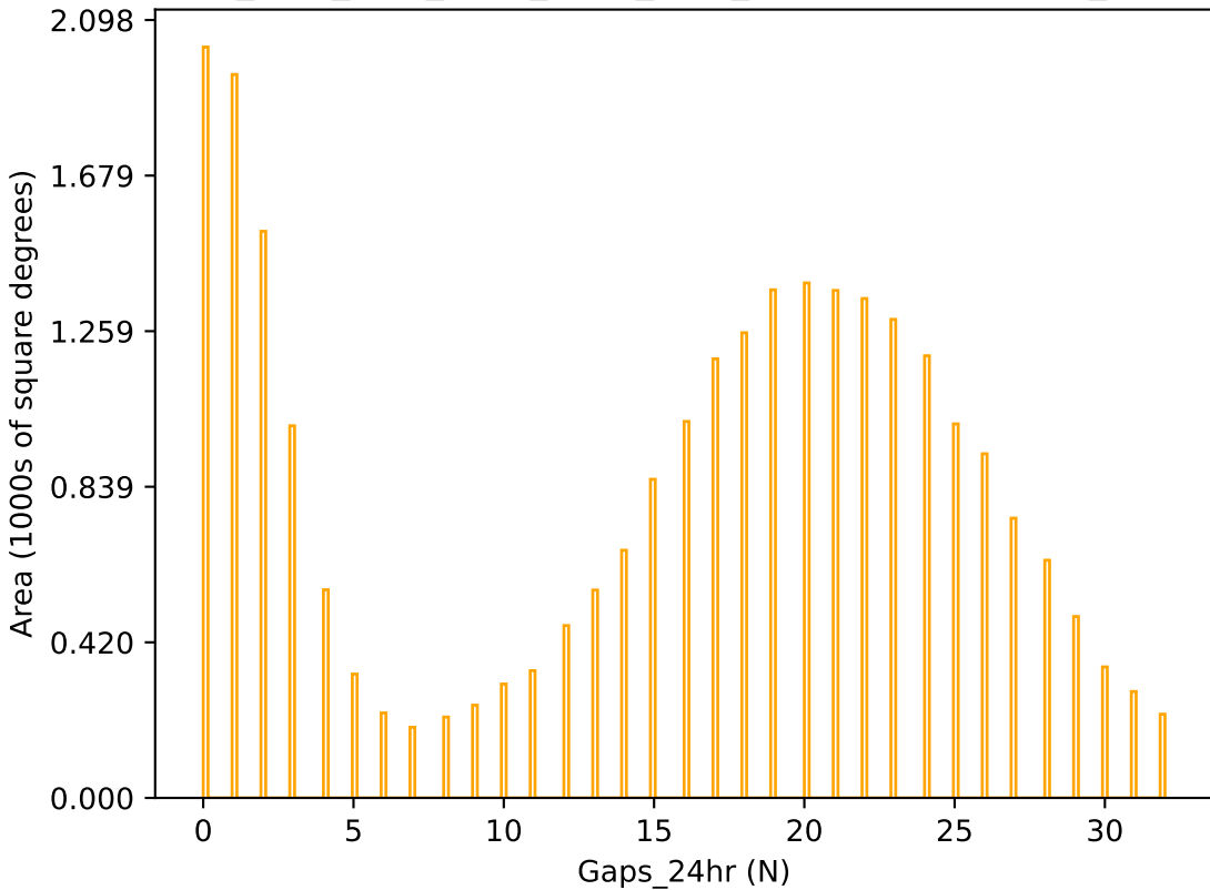
ddf_acor_sf20_lsf30_lsr20_v3.4_10yrs r band: Gaps_24hr
