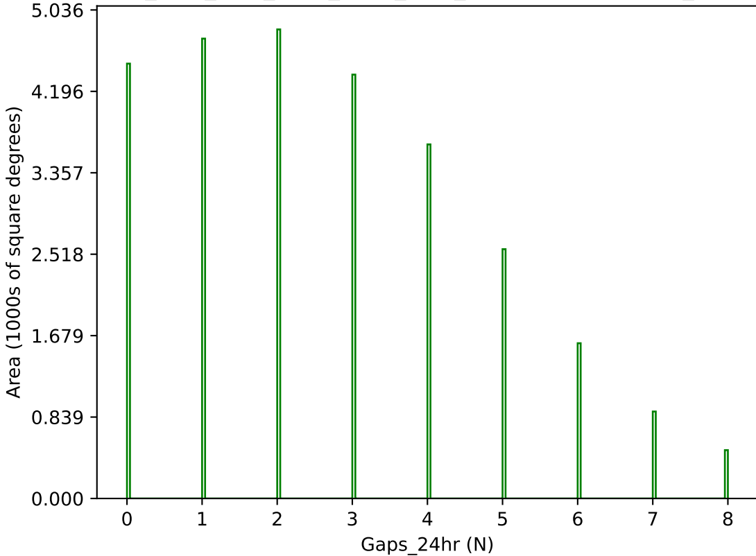
ddf_acor_sf20_lsf30_lsr20_v3.4_10yrs g band: Gaps_24hr
