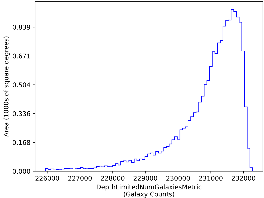
ddf_acor_sf20_lsf30_lsr20_v3.4_10yrs i band galaxies non-DD: DepthLimitedNumGalaxiesMetric
