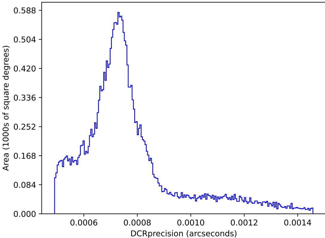
ddf_acor_sf20_ls30_lsr20_v3.4_10yrs : DCRprecision
