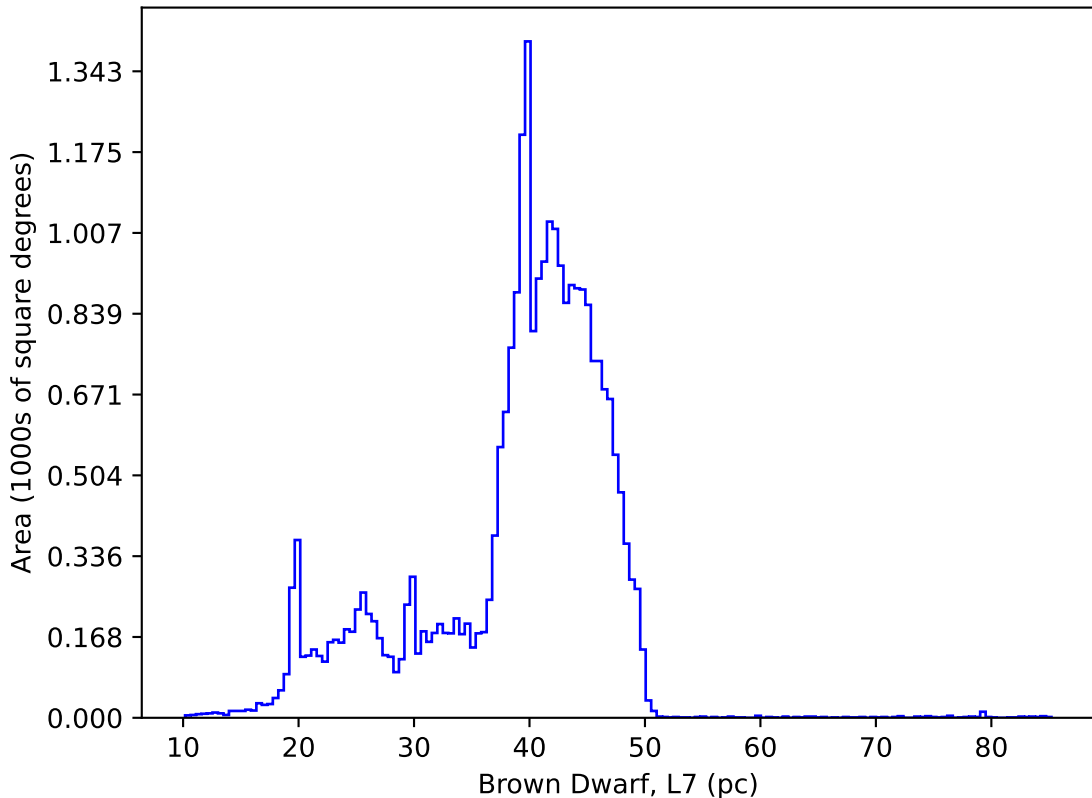
ddf_acor_sf20_lsf30_lsr20_v3.4_10yrs : Brown Dwarf, L7
