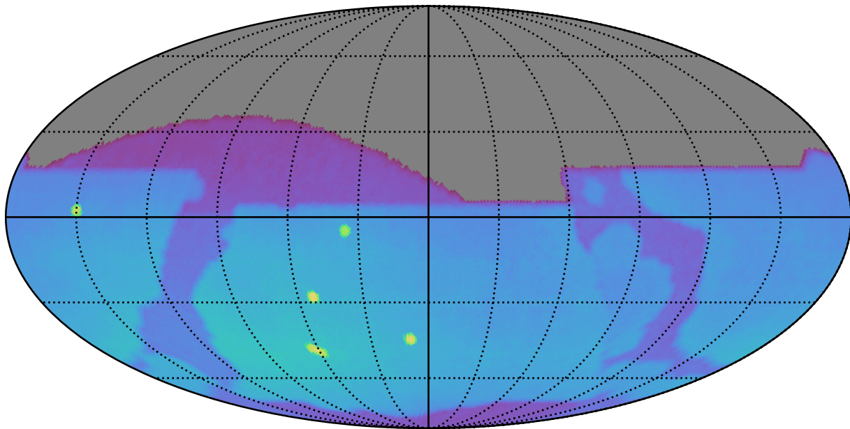
ddf_acor_sf20_lsf30_lsr20_v3.4_10yrs : Brown Dwarf, L4
