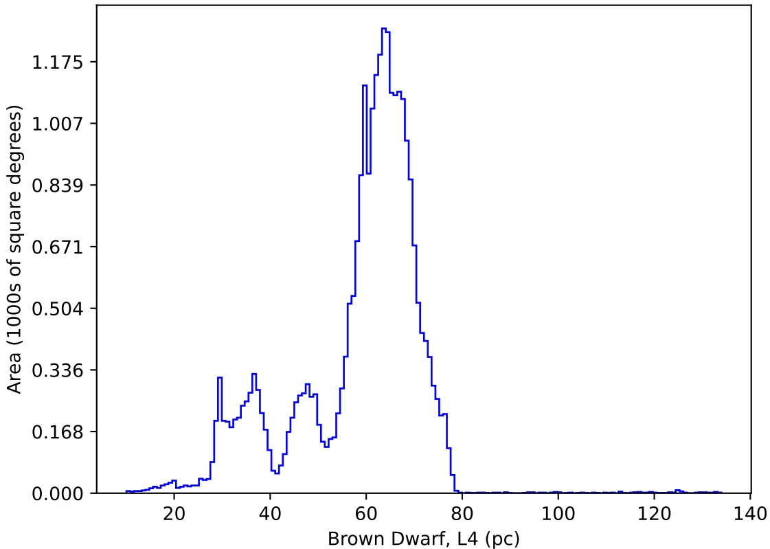
ddf_acor_sf20_lsf30_lsr20_v3.4_10yrs : Brown Dwarf, L4
