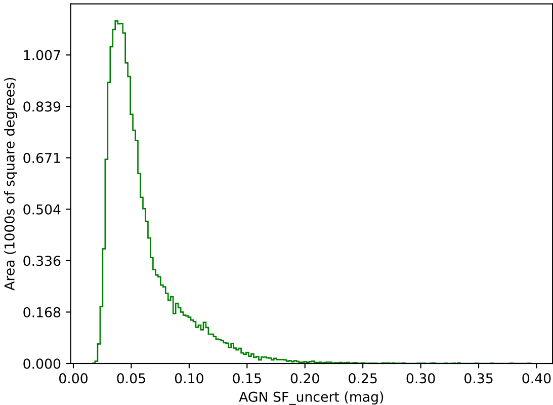
ddf_acor_sf20_lsf30_lsr20_v3.4_10yrs g band: AGN SF_uncert
