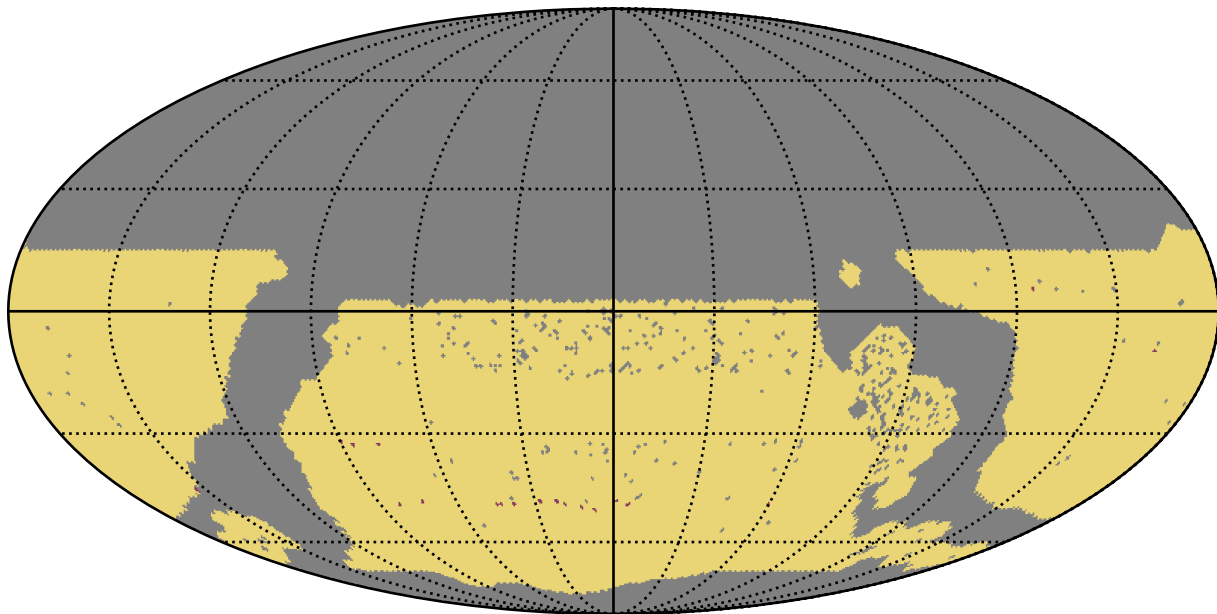
ddf_acor_sf20_lsf30_lsr20_v3.4_10yrs WFD: RapidRevisits
