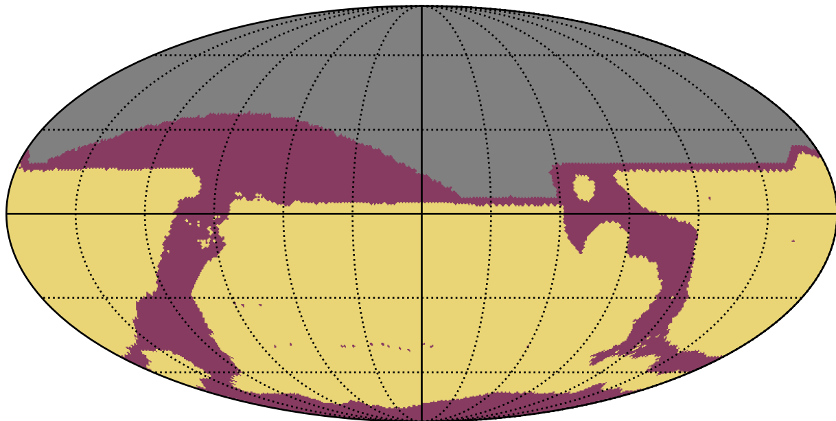
ddf_acor_sf20_lsf30_lsr20_v3.4_10yrs All sky: RapidRevisits
