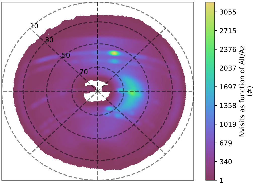
ddf_acor_sf20_lsf30_lsr20_v3.4_10yrs z band: Nvisits as function of Alt/Az
