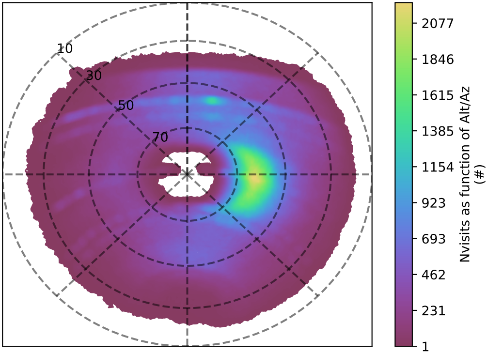
ddf_acor_sf20_lsf30_lsr20_v3.4_10yrs y band: Nvisits as function of Alt/Az
