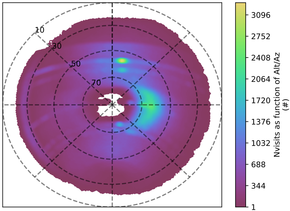
ddf_acor_sf20_lsf30_lsr20_v3.4_10yrs r band: Nvisits as function of Alt/Az
