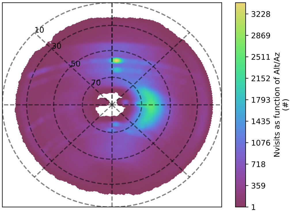
ddf_acor_sf20_lsf30_lsr20_v3.4_10yrs i band: Nvisits as function of Alt/Az
