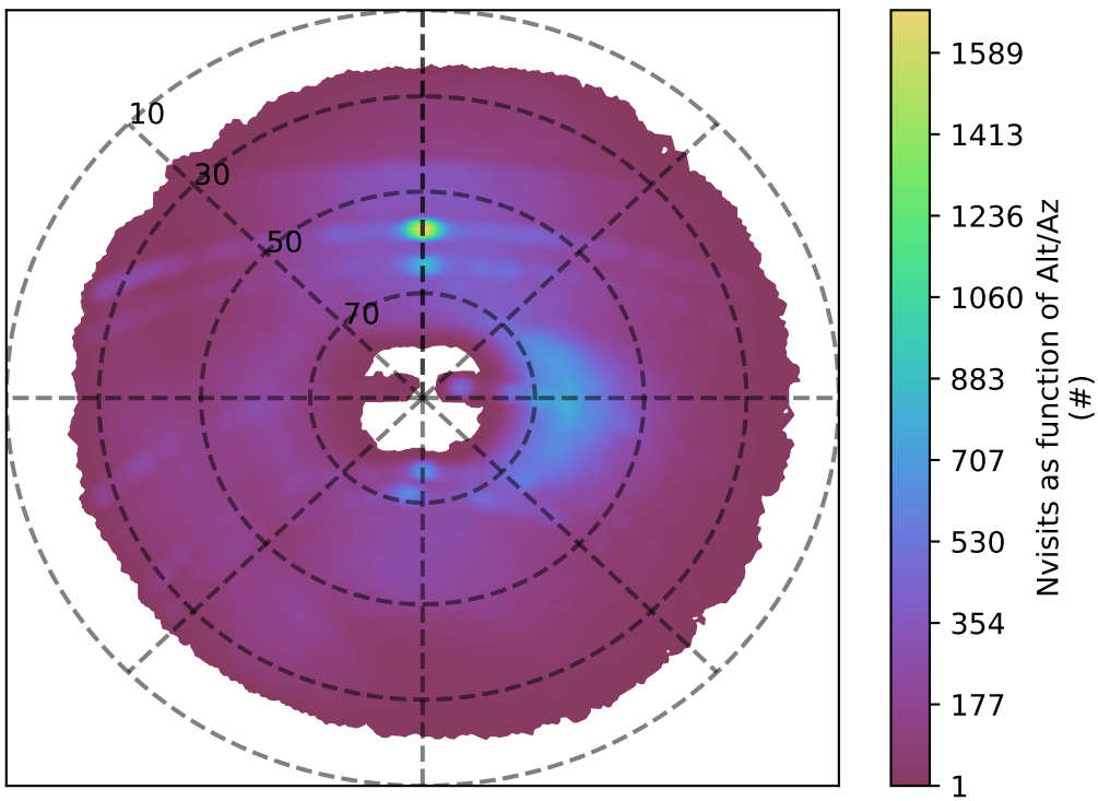
ddf_acor_sf20_lsf30_lsr20_v3.4_10yrs g band: Nvisits as function of Alt/Az
