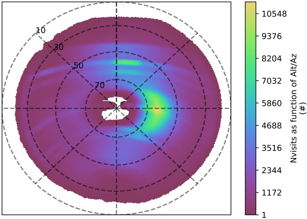
ddf_acor_sf20_ls30_lsr20_v3.4_10yrs all bands: Nvisits as function of Alt/Az
