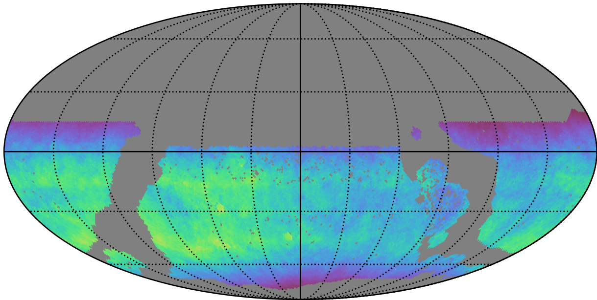
ddf_acor_sf20_lsf30_lsr20_v3.4_10yrs WFD y band: Normalized Teff
