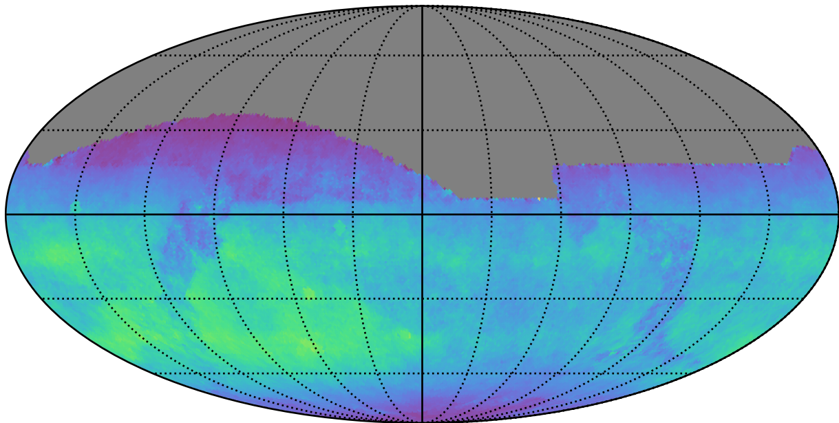
ddf_acor_sf20_lsf30_lsr20_v3.4_10yrs All sky z band: Normalized Teff
