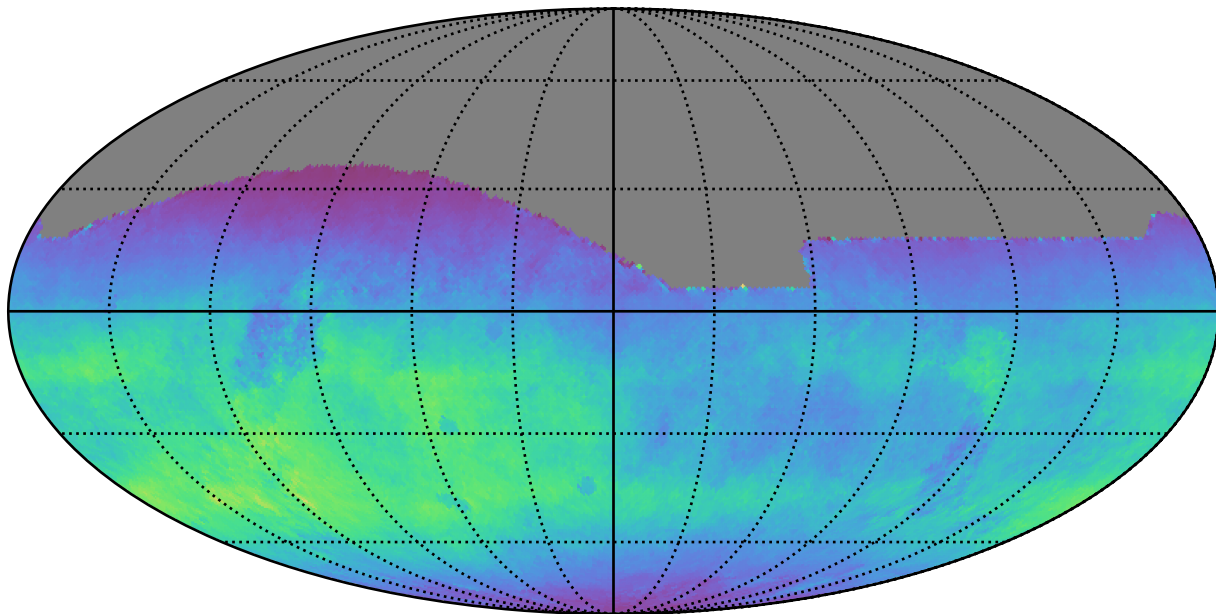
ddf_acor_sf20_lsf30_lsr20_v3.4_10yrs All sky r band: Normalized Teff
