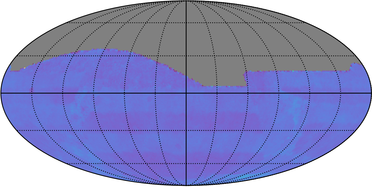
ddf_acor_sf20_lsf30_lsr20_v3.4_10yrs All sky: Normalized Proper Motion Uncert @ 24.0
