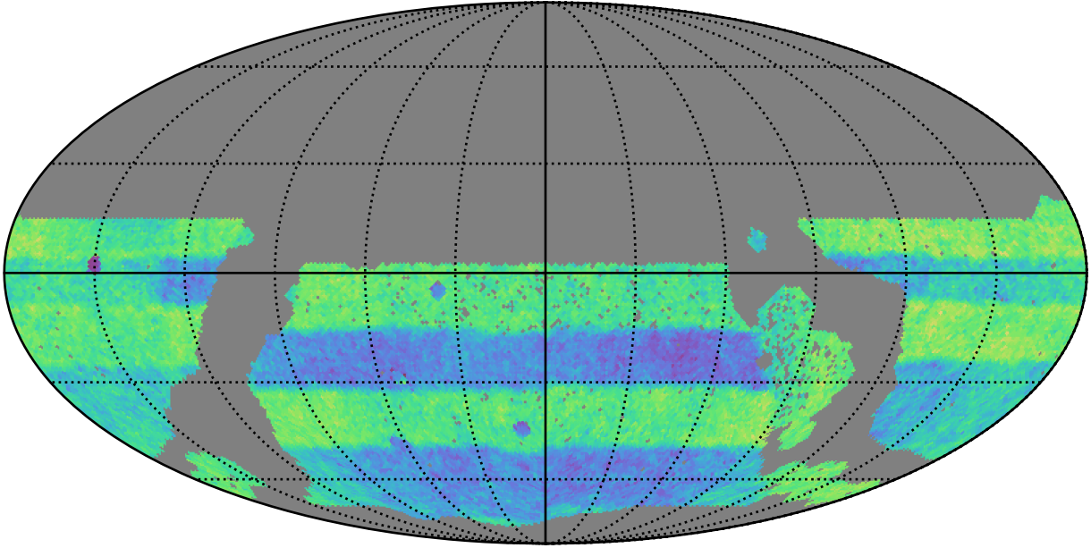
ddf_acor_sf20_lsf30_lsr20_v3.4_10yrs WFD: Normalized Proper Motion Uncert @ 20.5
