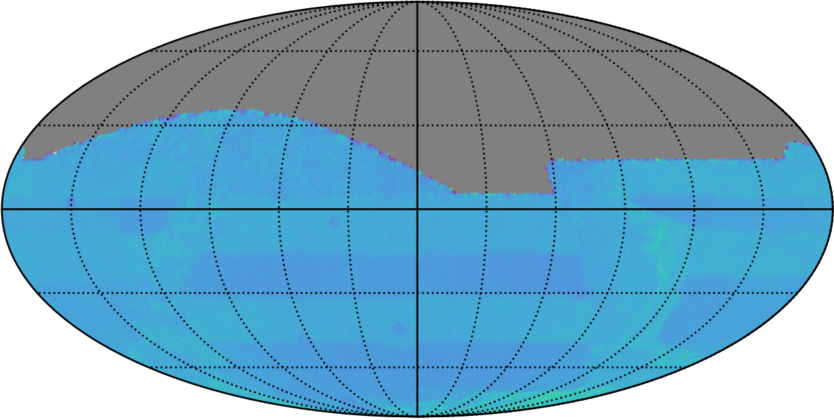
ddf_acor_sf20_lsf30_lsr20_v3.4_10yrs All sky: Normalized Proper Motion Uncert @ 20.5
