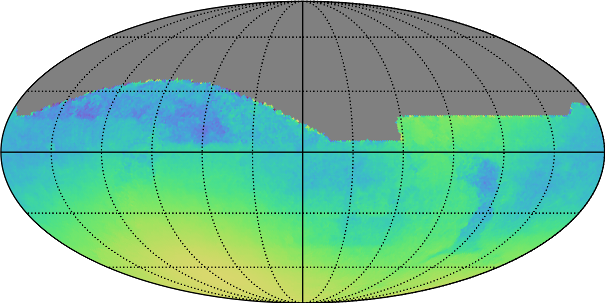
ddf_acor_sf20_lsf30_lsr20_v3.4_10yrs All sky: Normalized Parallax Uncert @ 24.0
