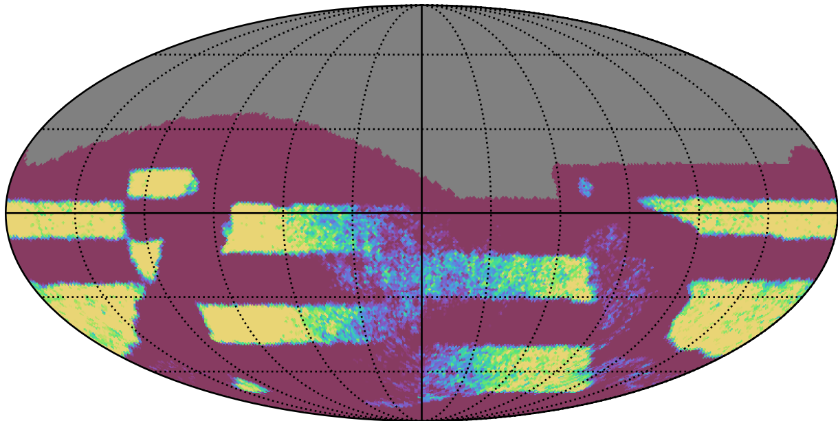
ddf_acor_sf20_lsf30_lsr20_v3.4_10yrs Yr 3-4 all bands: NVisits
