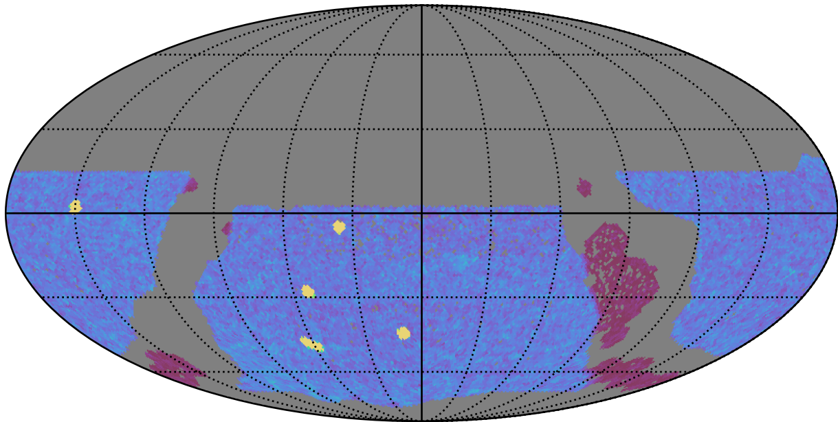
ddf_acor_sf20_lsf30_lsr20_v3.4_10yrs WFD y band: NVisits
