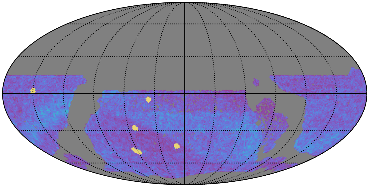
ddf_acor_sf20_lsf30_lsr20_v3.4_10yrs WFD all bands: NVisits
