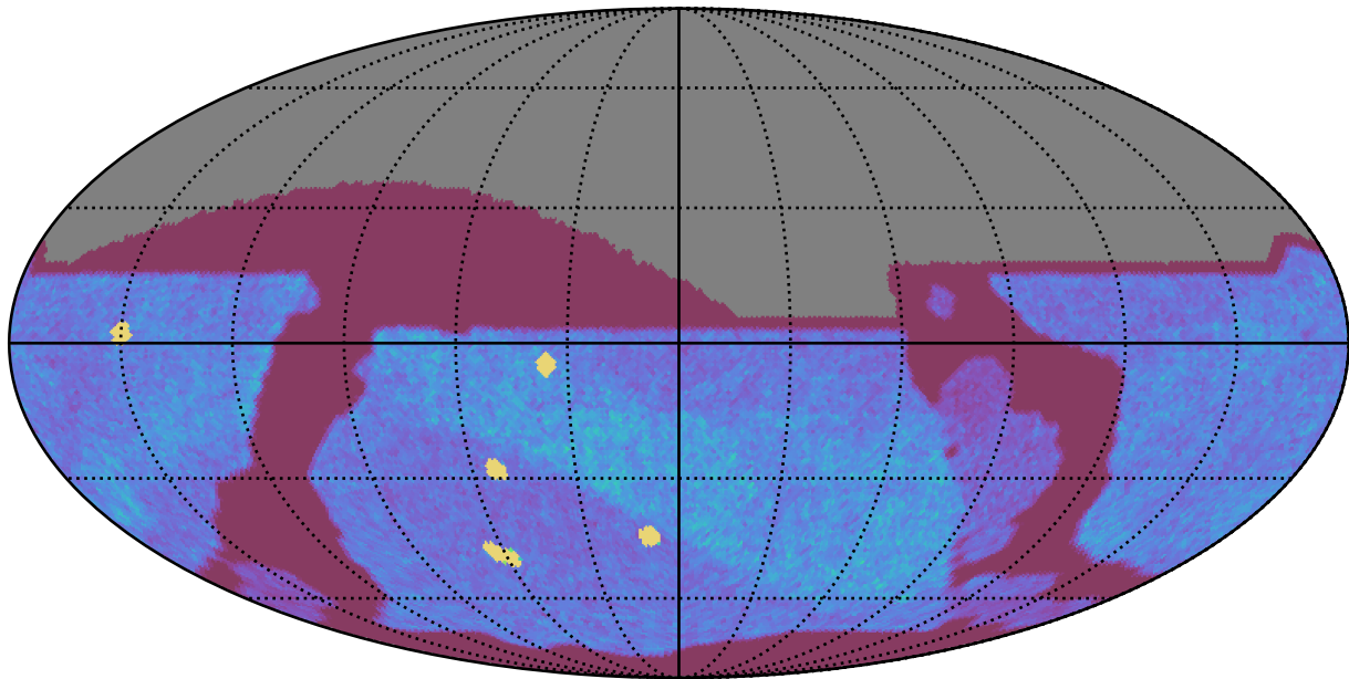
ddf_acor_sf20_lsf30_lsr20_v3.4_10yrs All sky z band: NVisits
