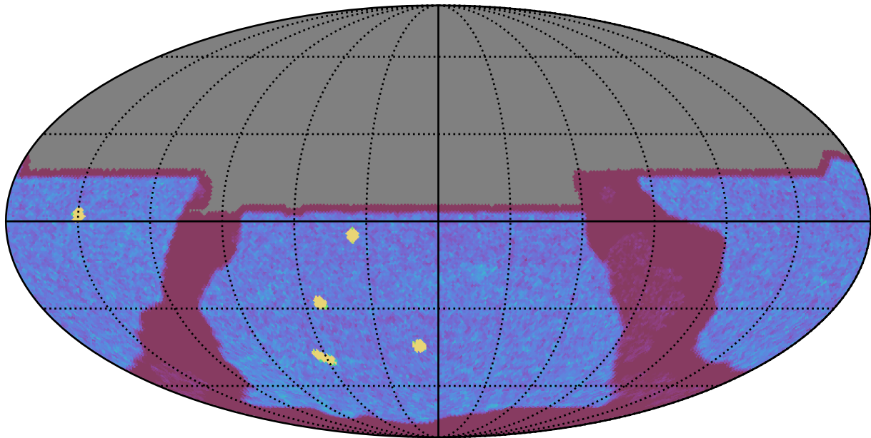
ddf_acor_sf20_lsf30_lsr20_v3.4_10yrs All sky y band: NVisits
